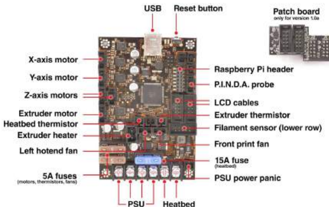
Pict. 42 - Proper wiring of the connectors
