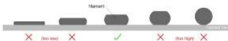
Pict. 10 - How to tune the nozzle height live during the test print. Note: -0.640 mm is only for illustration. Your setting will be different!
