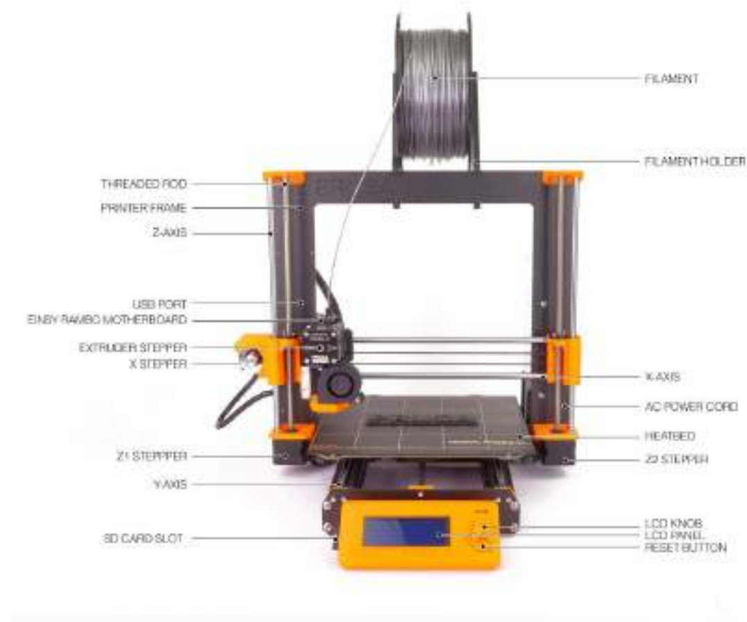
Pict. 1 - Original Prusa i3 MK3 printer description
