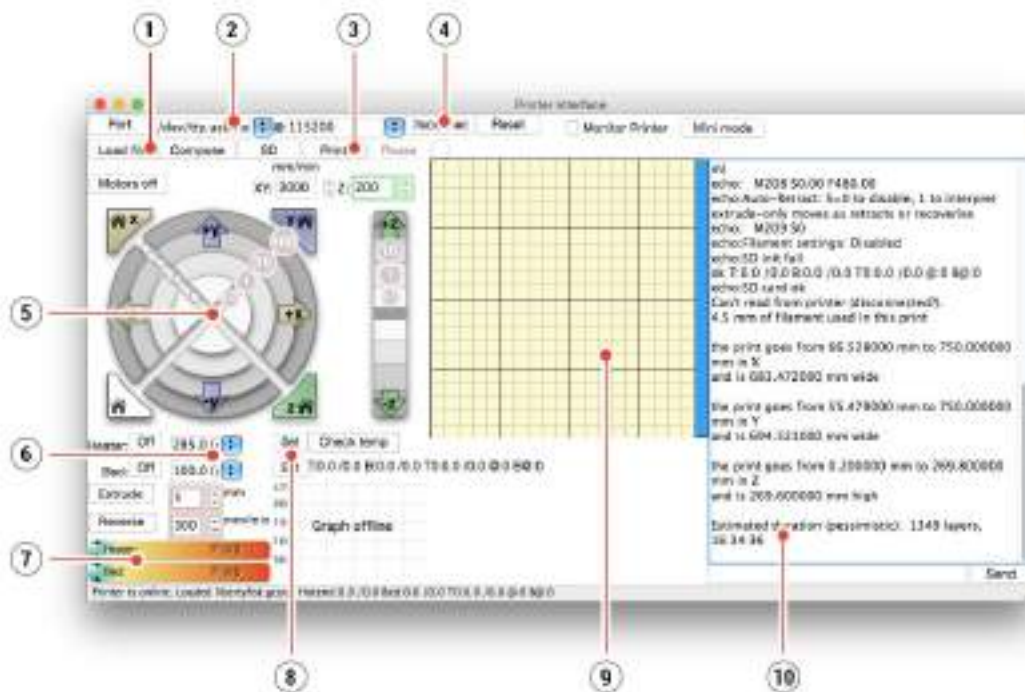
Pict. 22 - Pronterface
